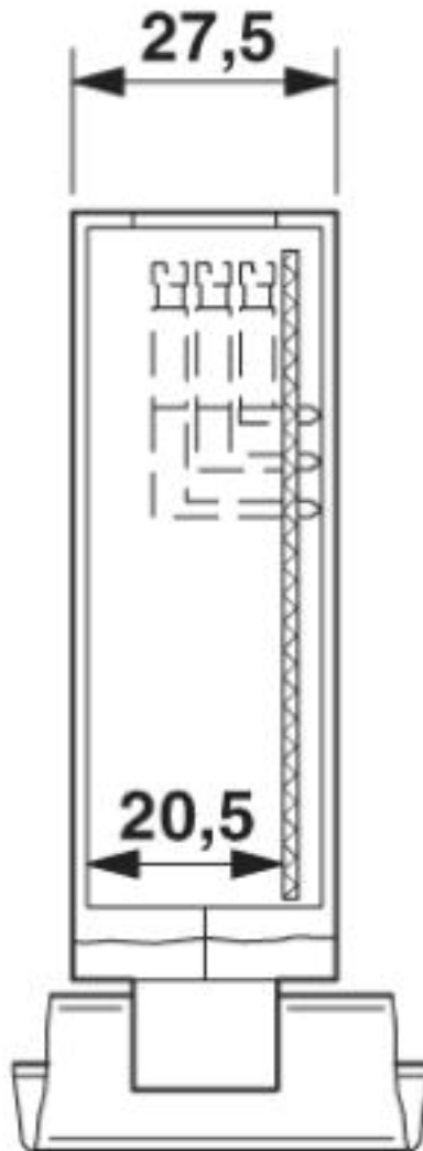
Dimensional drawing
