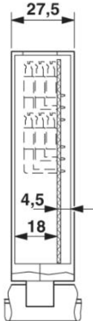
Dimensional drawing
