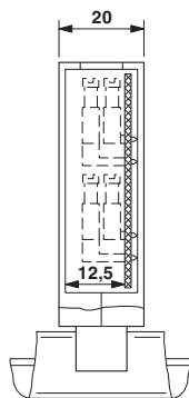
Dimensional drawing
