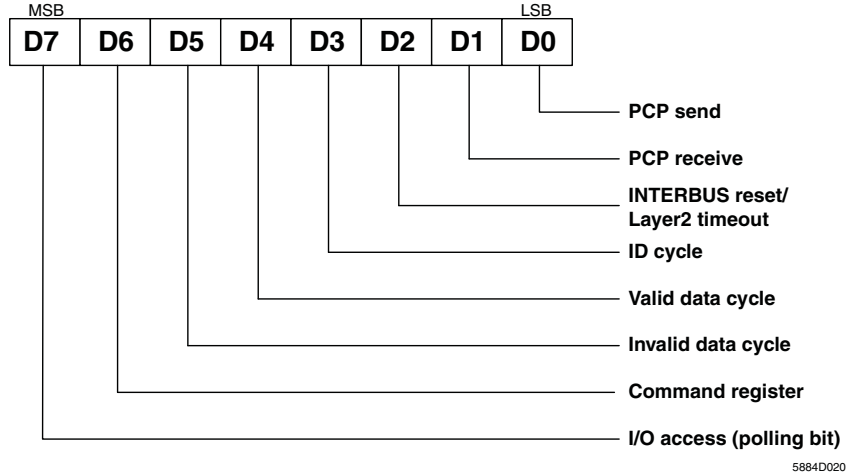
Figure 3-20 Interrupt event register assignment
