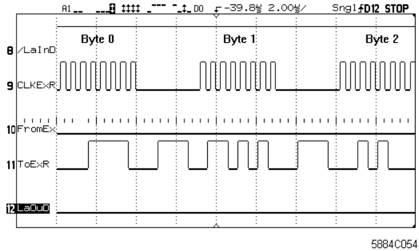
Figure 3-24 Assigning three data bytes with transmission via ToExR
