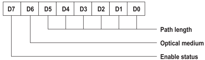
Figure 3-16 Length of the outgoing interface (READ register 8) and the bus branch (READ register 9)
