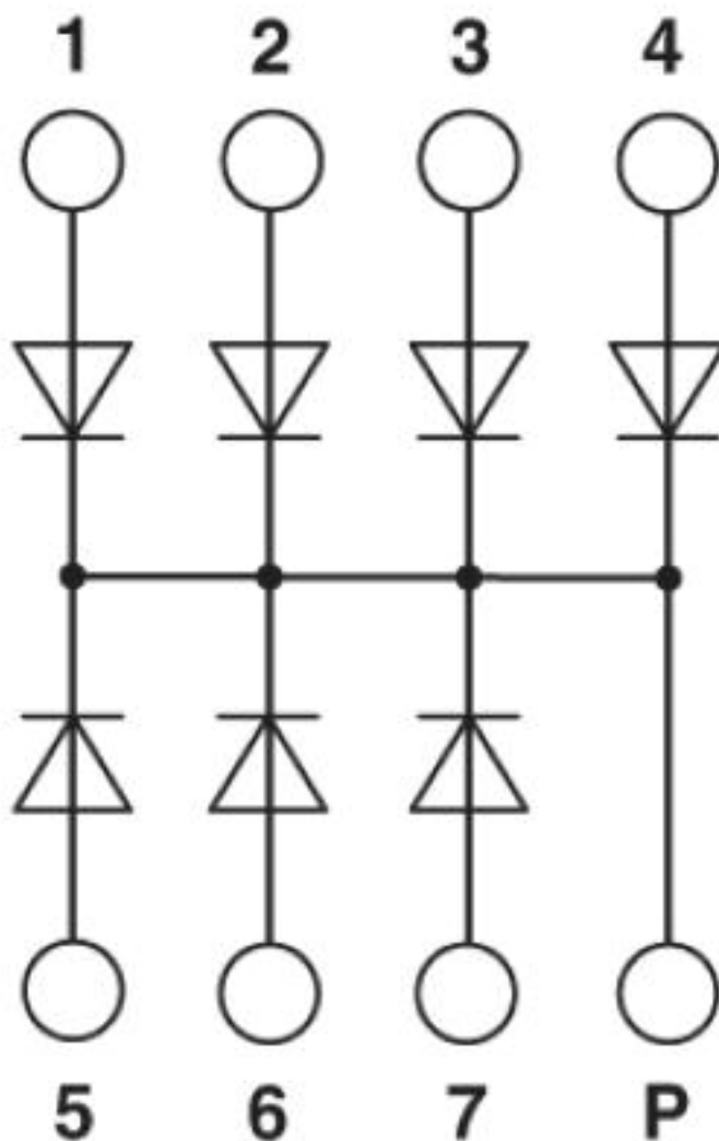
Circuit diagram
