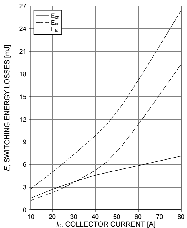
Figure 12. Typical switching energy losses as a function of collector current (inductive load, T_{vj}=175^{\circ}\text{C} , V_{CE}=600\text{V} , V_{GE}=15/0\text{V} , r_G=12\Omega , Dynamic test circuit in Figure E)
