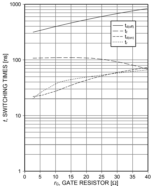
Figure 9. Typical switching times as a function of gate resistor (inductive load, T_{vj}=175^{\circ}\text{C} , V_{CE}=600\text{V} , V_{GE}=15/0\text{V} , I_C=40\text{A} , Dynamic test circuit in Figure E)
