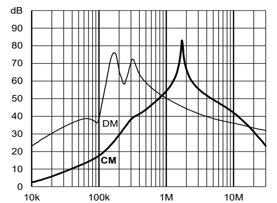
FN3288-230-40-C17-R65
