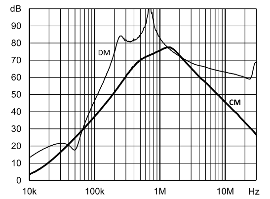
FN3288-50-53-C21-R65
