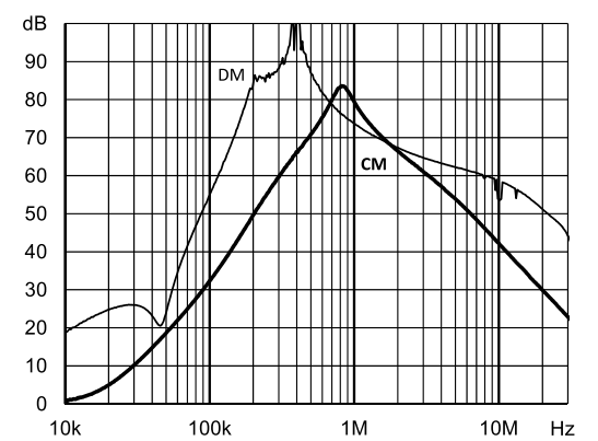
FN3288-100-35-C21-R65
