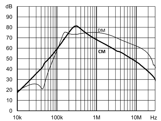
FN3288-100-35-C35-R65
