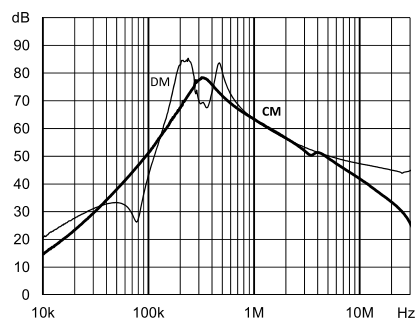
FN 3288-160-40-C35-R65
