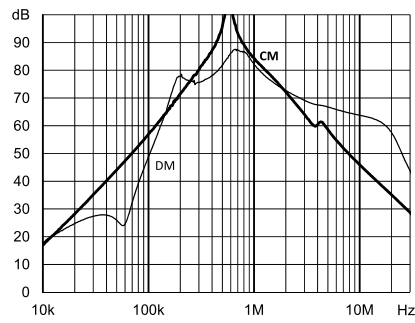
FN 3288-80-34-C35-R65
