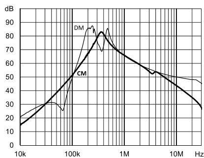
FN 3288-125-35-C35-R65
