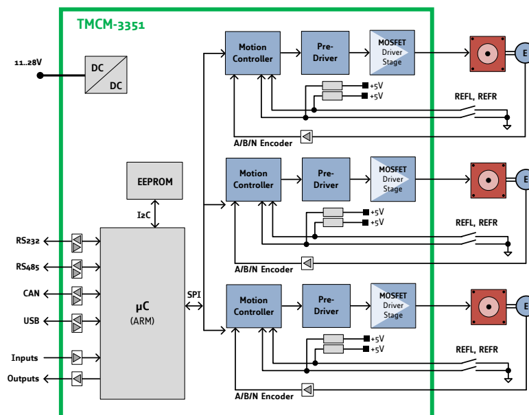
Figure 10: TMC3351 block diagram
