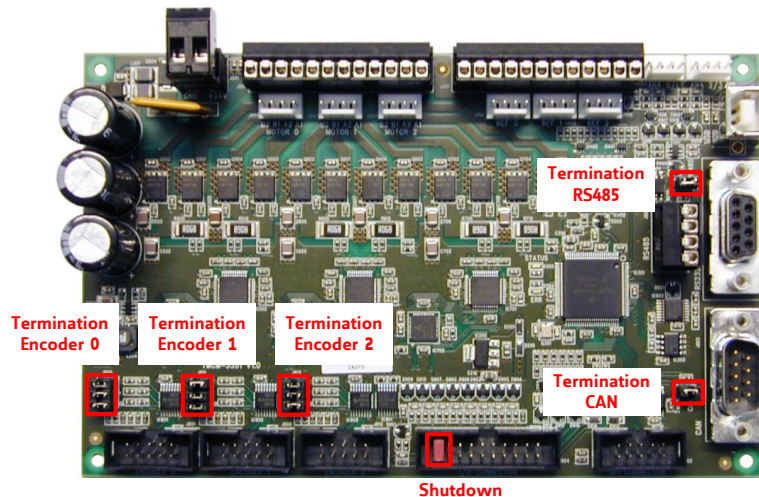
Figure 3: Jumper settings of TMC3351
