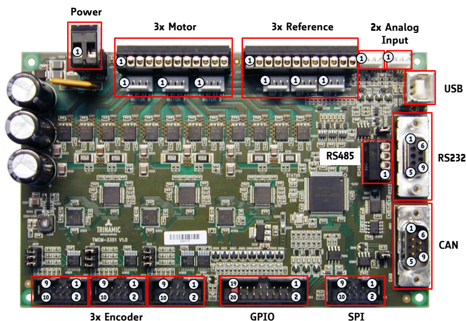
Figure 2: TMCM-3351 connectors
