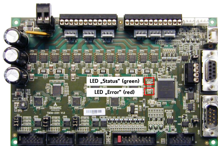
Figure 6: TMC3351 LEDs
