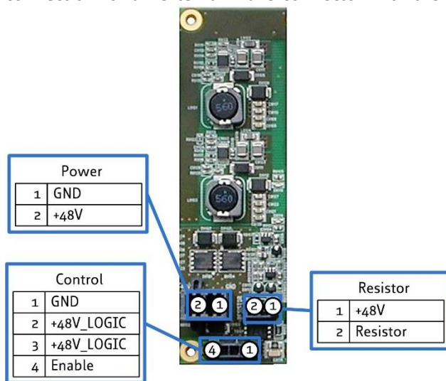
Figure 5.5: TMC314 + TMC315 Power supply Brick
