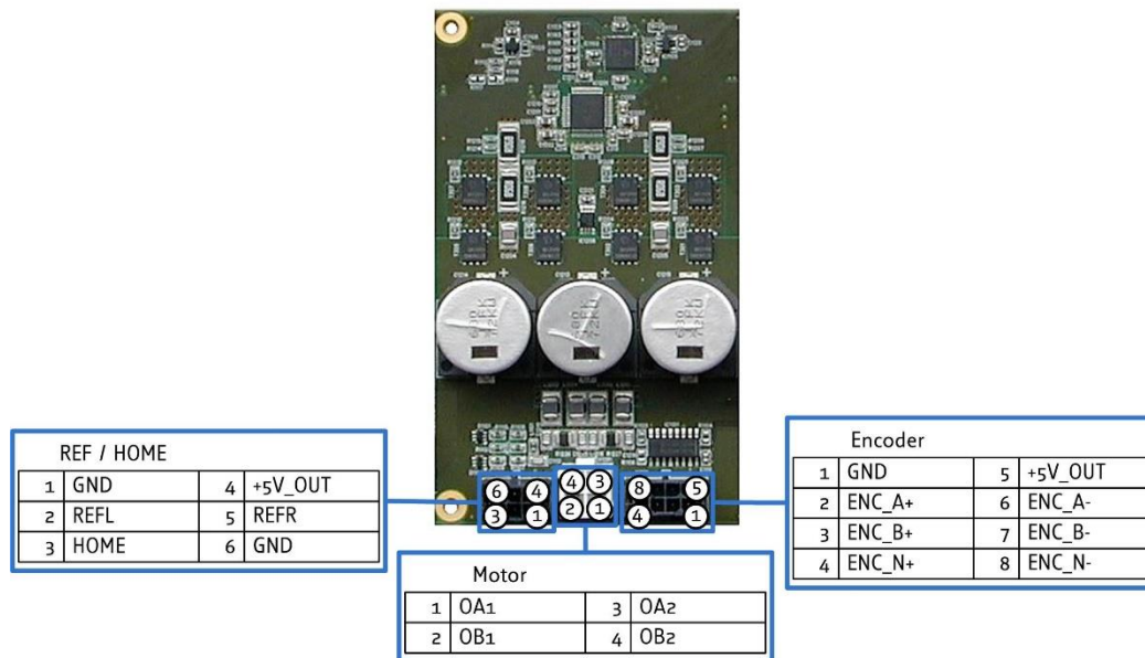
Figure 5.4 TMC314 + TMC315 Driver Brick
