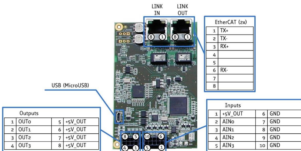
Figure 5.3 TMC315 interface brick
