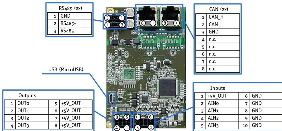
Figure 5.2 TMC314 interface brick
