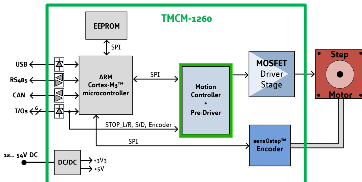
Figure 14: TMC-1260 block diagram
