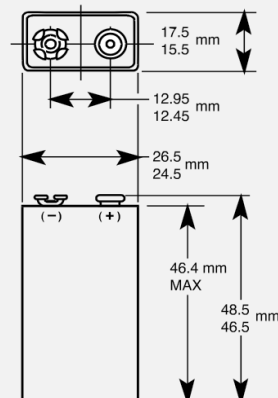
Dimensions shown are IEC standards
