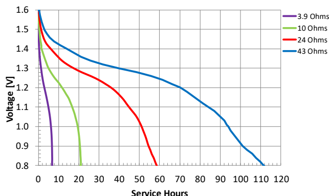
Constant Resistance
