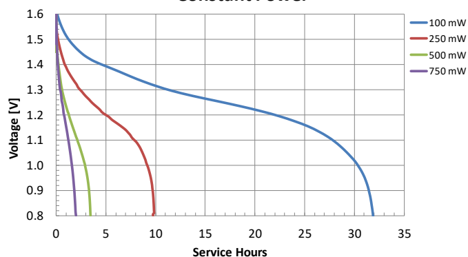
Constant Power
