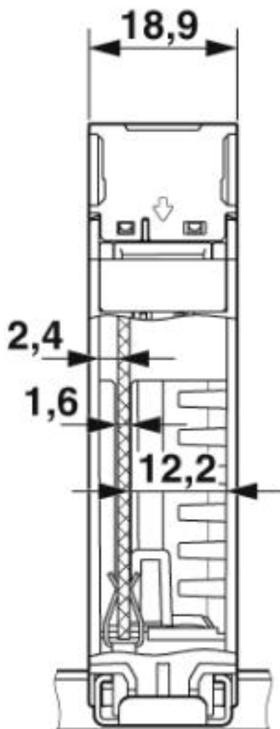
Dimensional drawing
