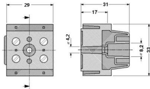
Dimensioned drawing
