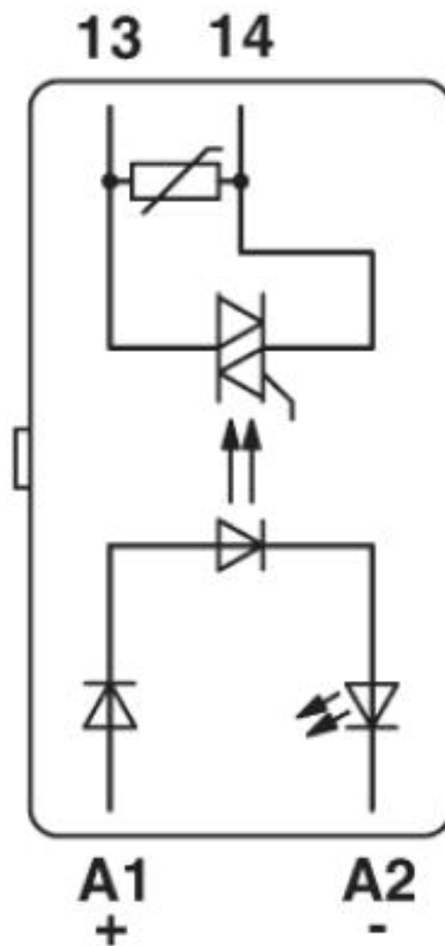
Circuit diagram
