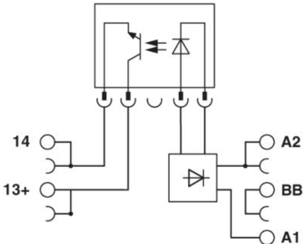
Circuit diagram
