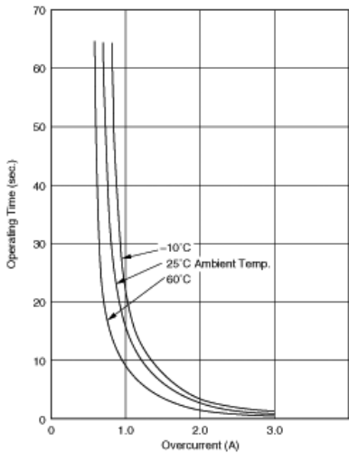
Operating Time (Typical Curve)
