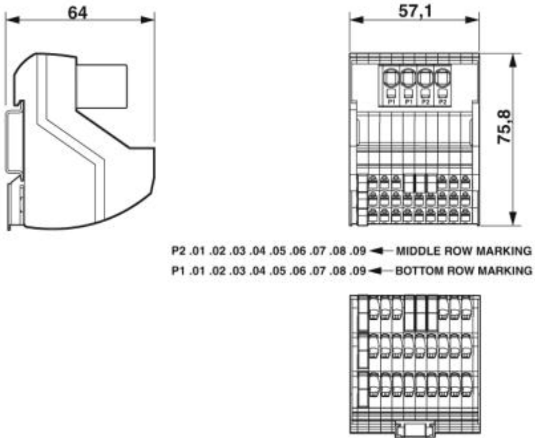
Dimensional drawing
