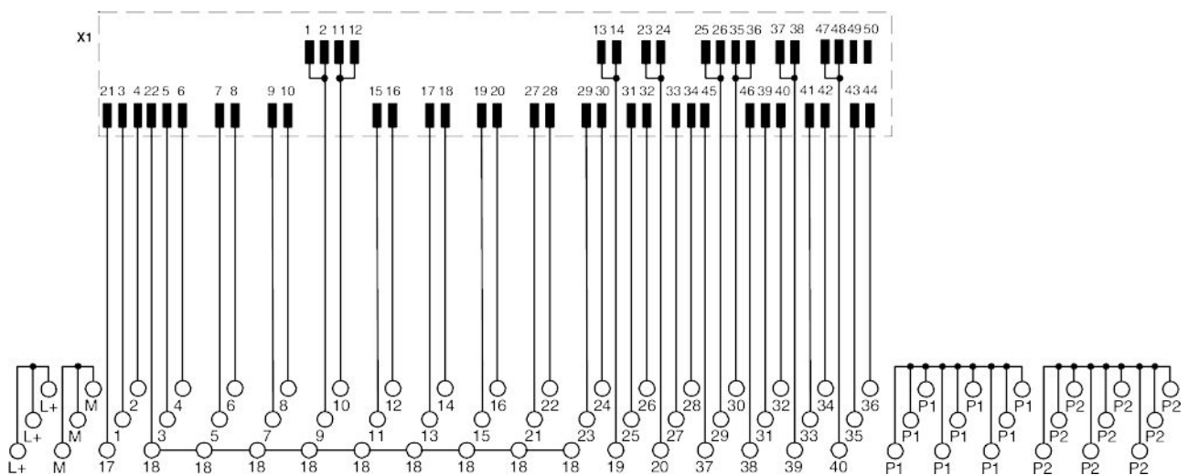
Circuit diagram
