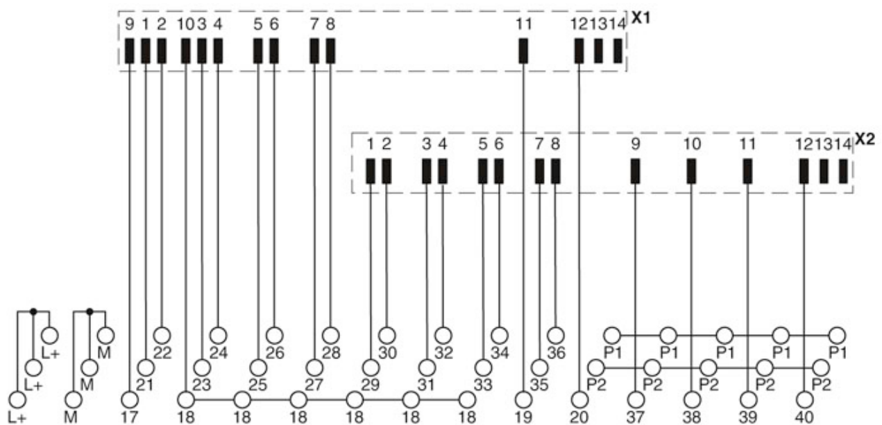
Circuit diagram
