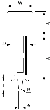
TERMINAL STYLE 1 (SINGLE PIN)
