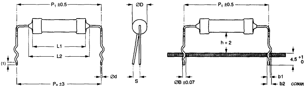
Dimensions in mm. For dimensions see Tables 4 and 6. (1) \varnothing 0.8 to 1.4 or \varnothing 0.6 to 1.6.
