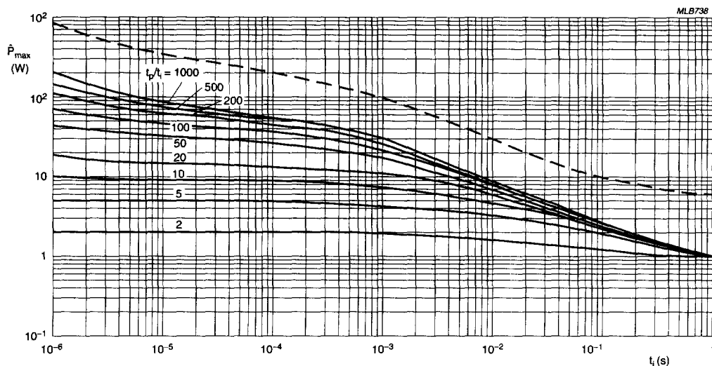
Fig.5 Pulse on a regular basis; maximum permissible peak pulse power ( \hat{P}_{max} ) as a function of pulse duration ( t_i ).
