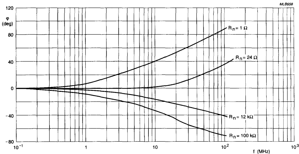
Fig.35 Phase angle as a function of applied frequency.
