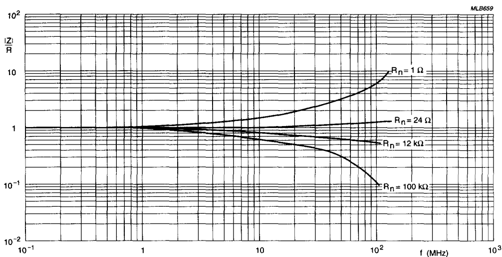
Fig.34 Impedance as a function of applied frequency.
