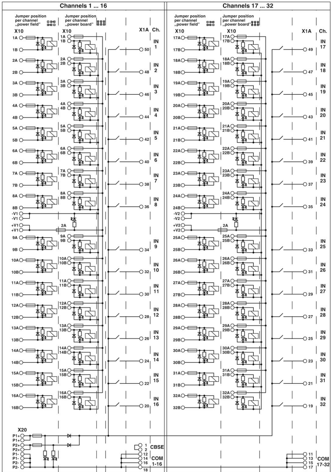
Circuit diagram
