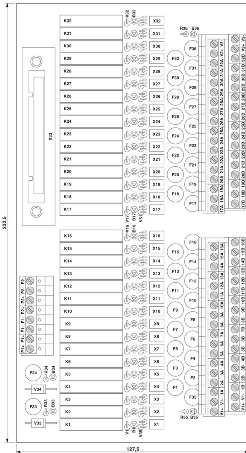
Dimensional drawing
