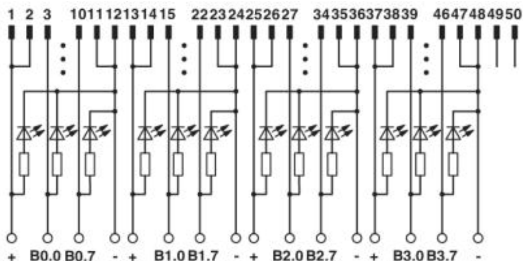
UM 45-FLK50/LA/PLC connection scheme
