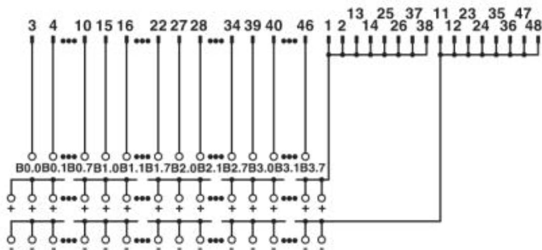
UM 45-FLK50/32IM/PLC connection scheme
