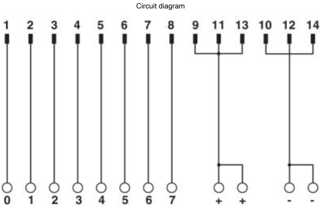
UM 45-FLK14/ZFKDS/PLC connection scheme
