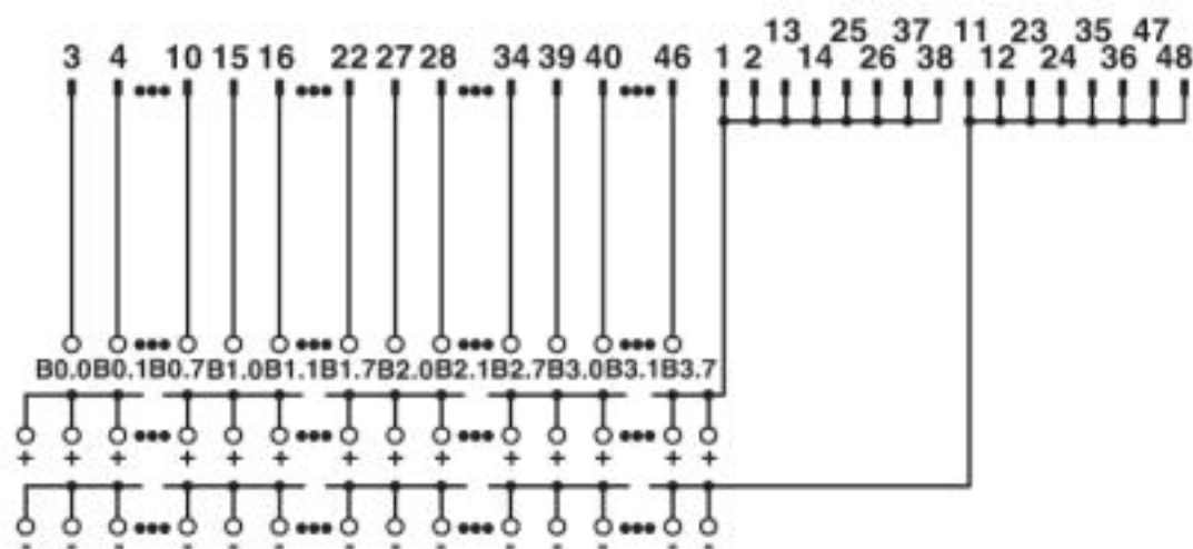
Connection scheme FLKMS 50/32IM/PLC
