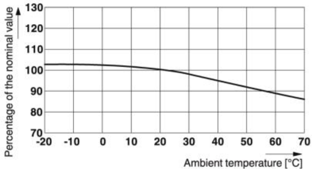
TR5 fuse derating curve
