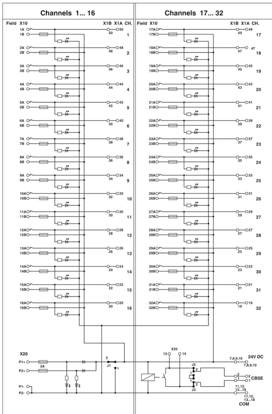
Circuit diagram
