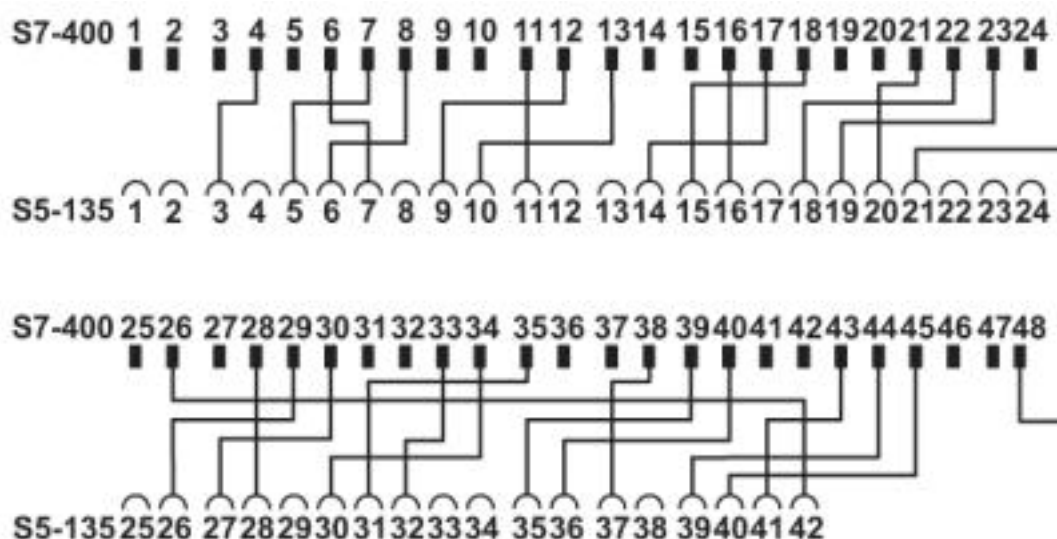
Connection scheme FLKM S135-470-4UC/I/S400
