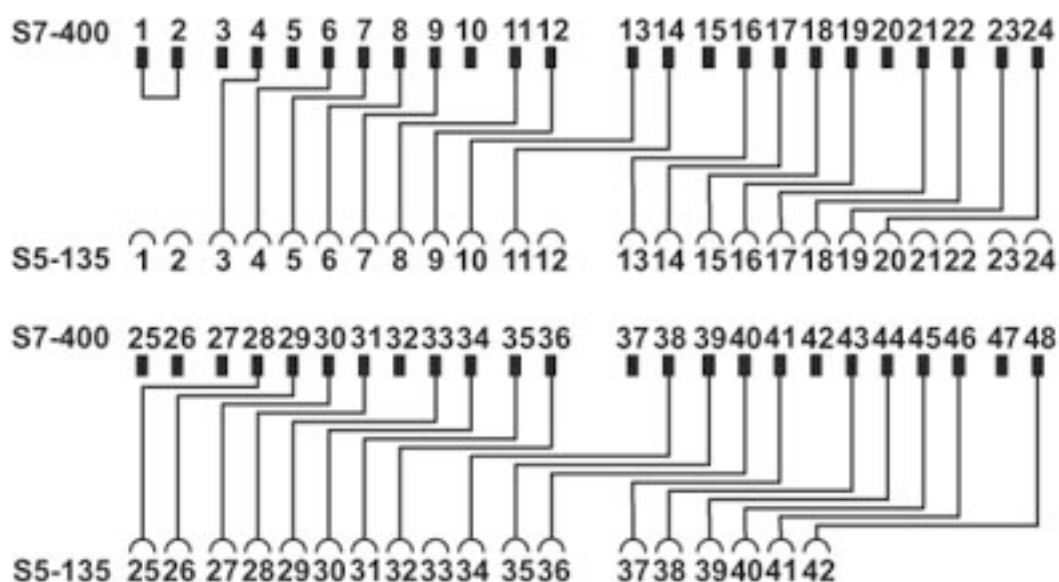
FLKM S135-465-4UA/UI/S400 connection scheme
