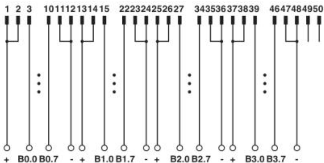
Connection scheme FLKM 50/PLC
