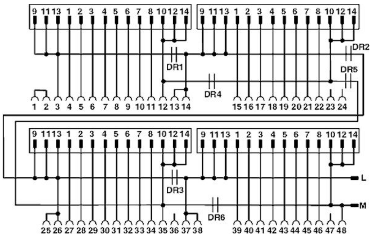
Circuit diagram
