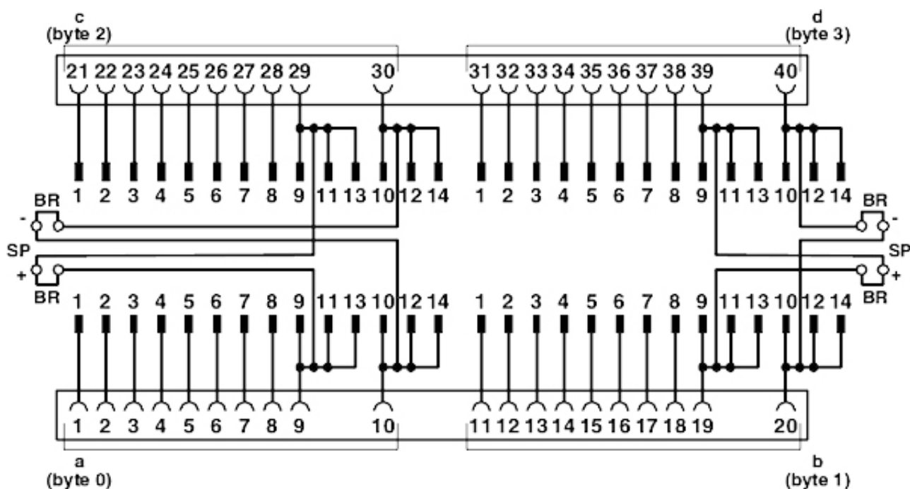
Circuit diagram
