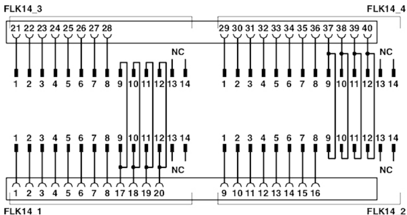
Circuit diagram
