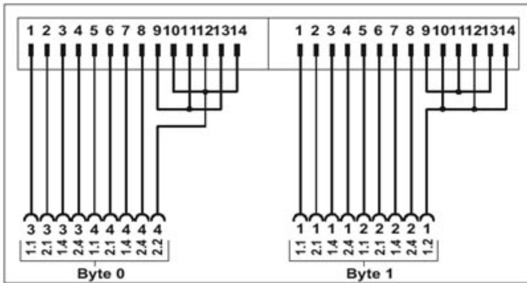
Connection diagram
