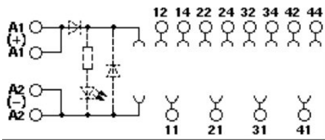
Circuit diagram
