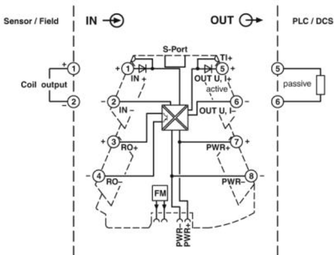
Block diagram
