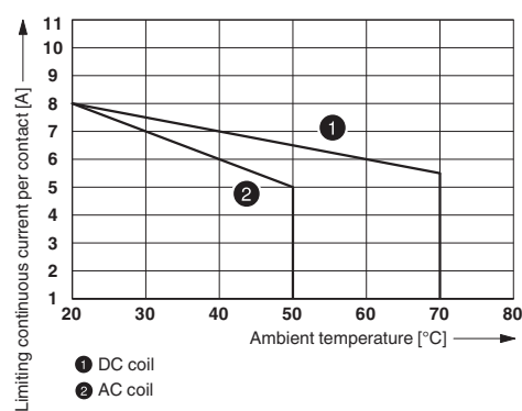
Contact derating
