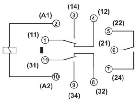
Circuit diagram
