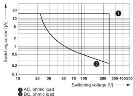
Interrupting rating
