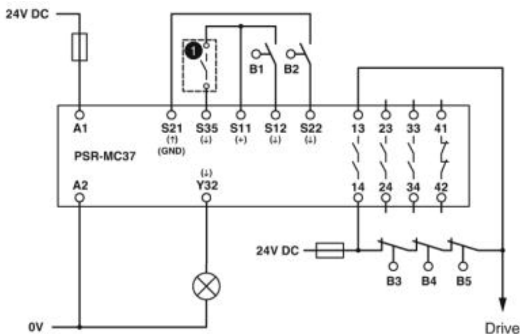
Circuit diagram
