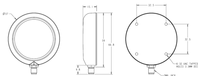
Dimensions (mm)
