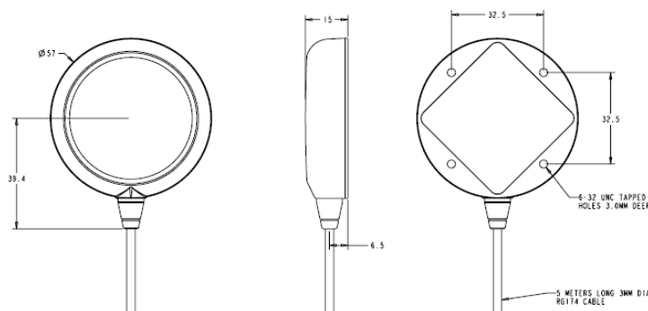
Dimensions (mm)
