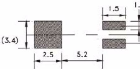
Recommended Land Pattern
