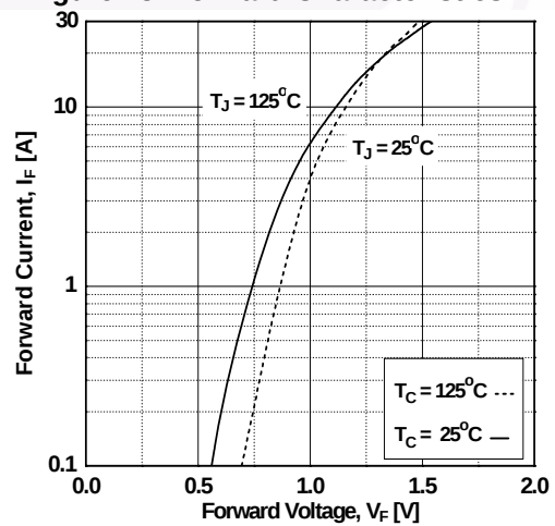
Figure 18. Forward Characteristics
