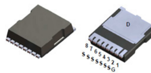
H-PSOF8L CASE 100CU
