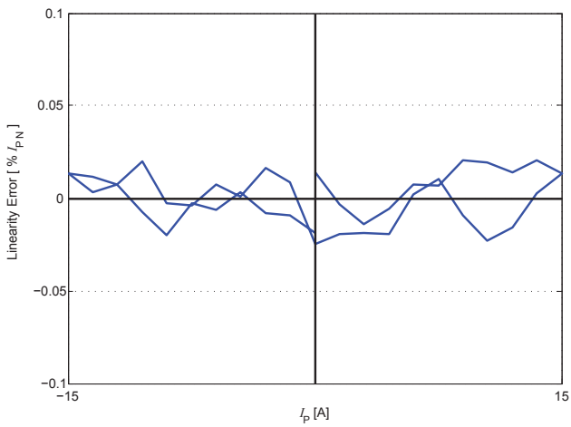
Figure 6: Linearity error
