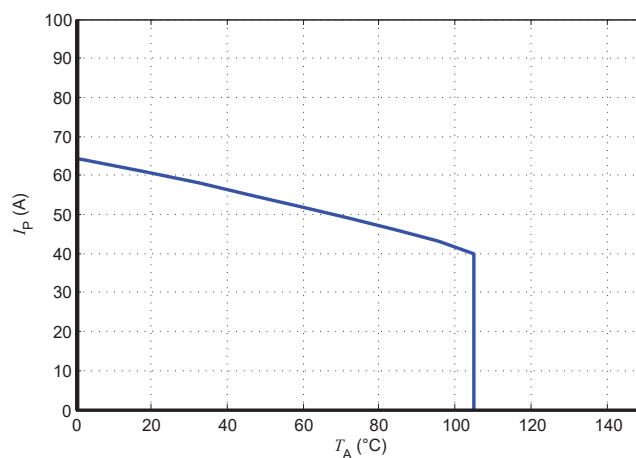
Figure 17: I_p vs T_A for LXS 15-NPS
