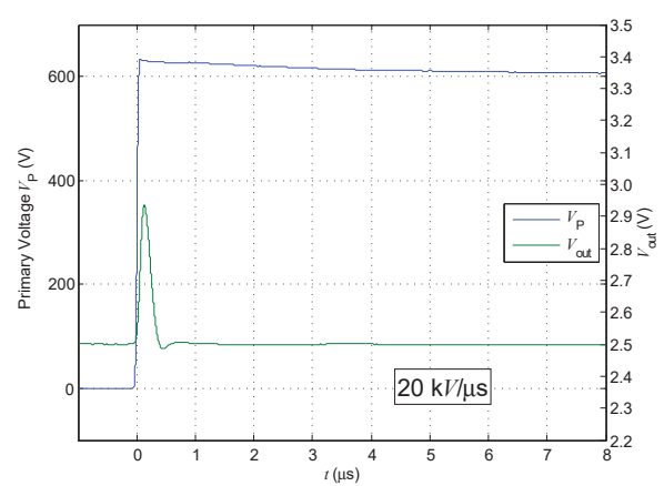
Figure 5: dv/dt
