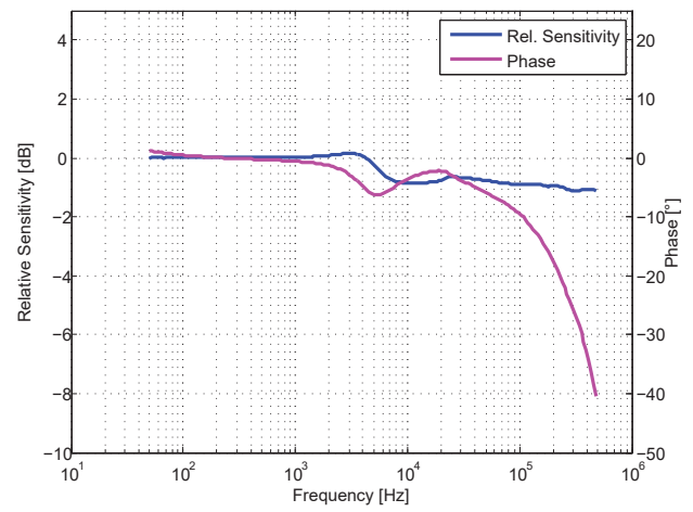
Figure 7: Frequency response
