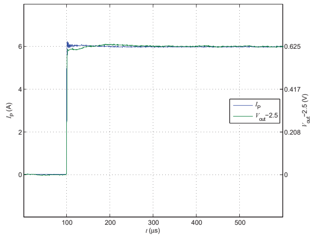
Figure 3: Step response
