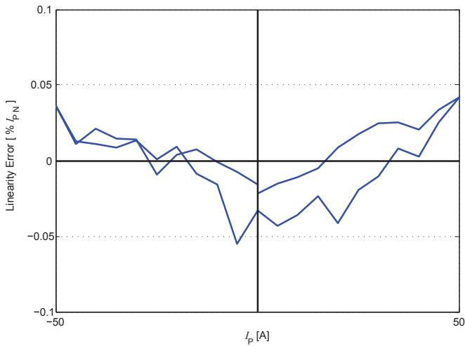
Figure 16: Linearity error
