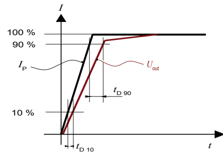
Figure 3: t_{D10} (delay time @ 10 %) and t_{D90} (delay time @ 90 %)
